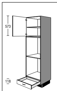
1907 mm SNK 7060 600
